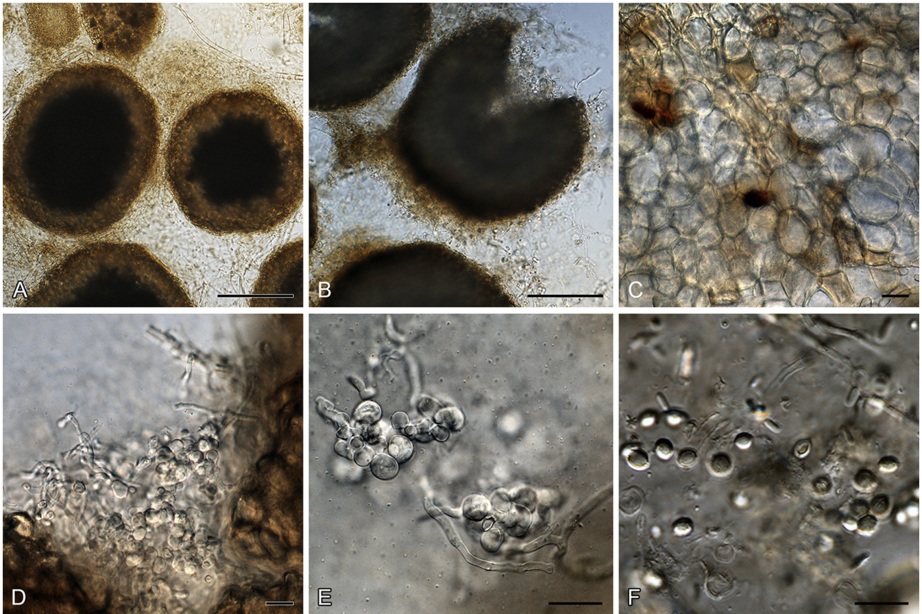
Fig. 4. Penicillium paradoxum sexual reproduction. A–C. Cleistothecia. D, E. Asci. F. Ascospores. Scale bars: A, B = 500 \mu m; C–F = 10 \mu m.
