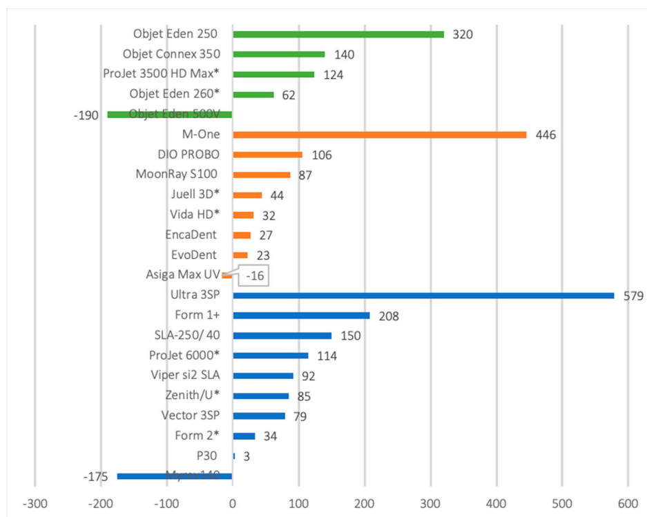
Figure 2. Reported trueness in microns for material jetting (MJ, green), digital light processing (DLP, orange) and stereolithography (SLA, blue) 3D printed full-arch dental models. * Asterisk denotes lowest mean error identified from different studies—other results in microns reported include: Form 2 = 59, 64 and −80; Zenith series = 138; ProJet 6000 = 190; Juell 3D = 44, 70; Vida = 56; Objet Eden 260 series = 74, 80 and 85; ProJet 3500 HD Max = 129. Data from studies that did not report details of 3D printer used or trueness data were not included in the figure.
