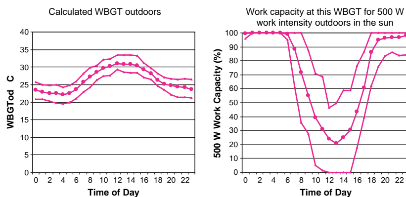
Fig. 1. Calculated WBGT outdoors in the sun and resulting work capacity at 500 W work intensity during different hours of a 24-hour period in Delhi, India, May 1999 (based on hourly weather data from the NOAA database; the middle line is the monthly mean, the other lines the 5 and 95 percentiles of recordings on individual days during that month).
